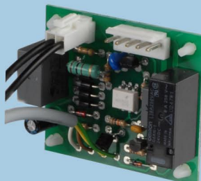
Electronic card
