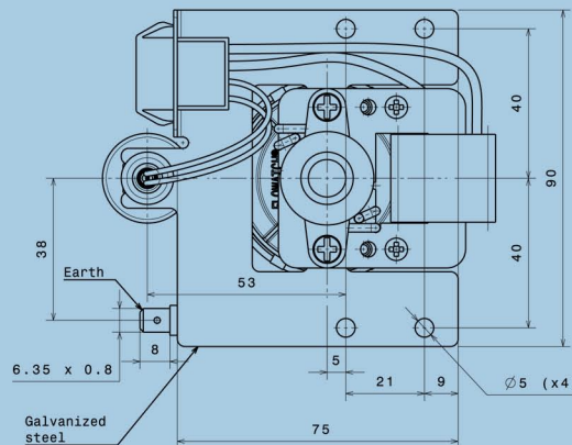
Drawing CP08 Pack alarm
